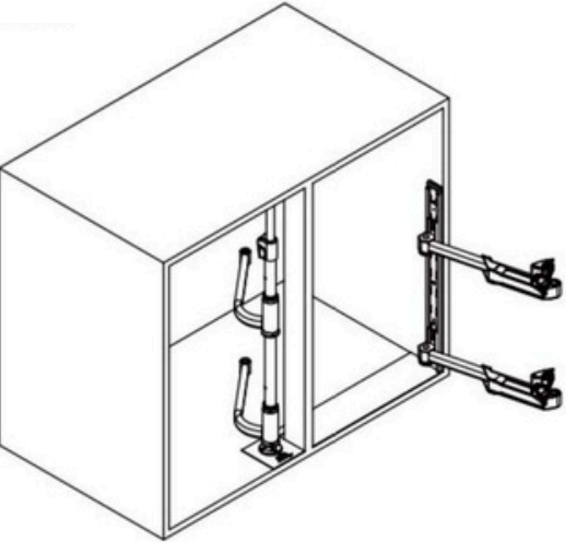
Diagram Instalasi
